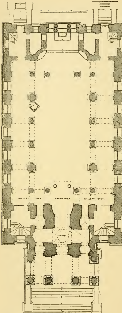
PLAN OF CHRIST CHURCH, SPITALFIELDS.
